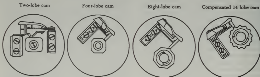
FIGURE 4-8. Typical breaker assemblies.
